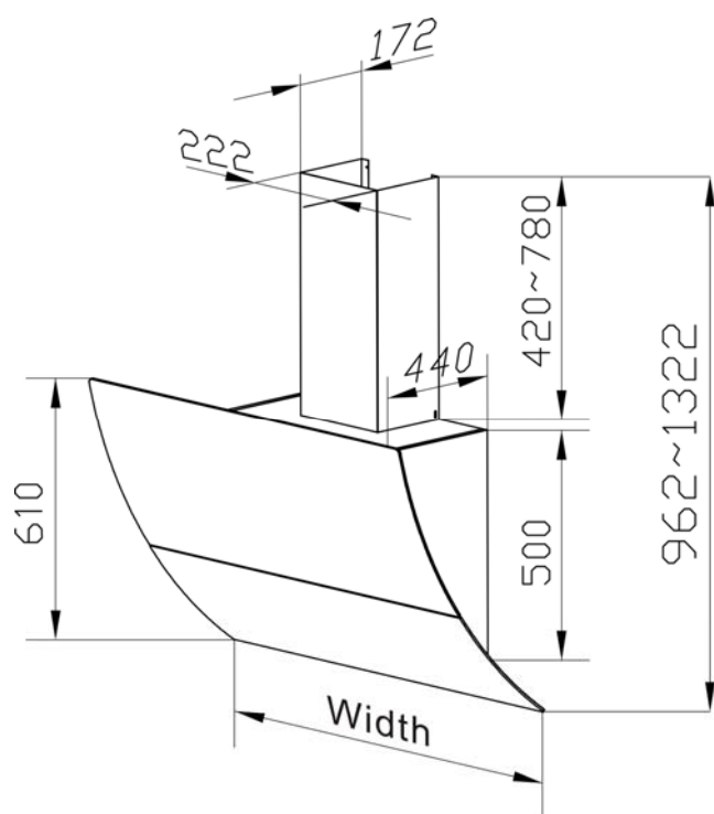
BDR603TFG, BDR603TFG-F, Width=600;
