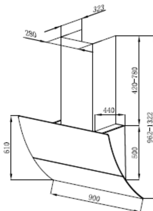
BDR903TFG, BDR903TFG-F, Width=900
